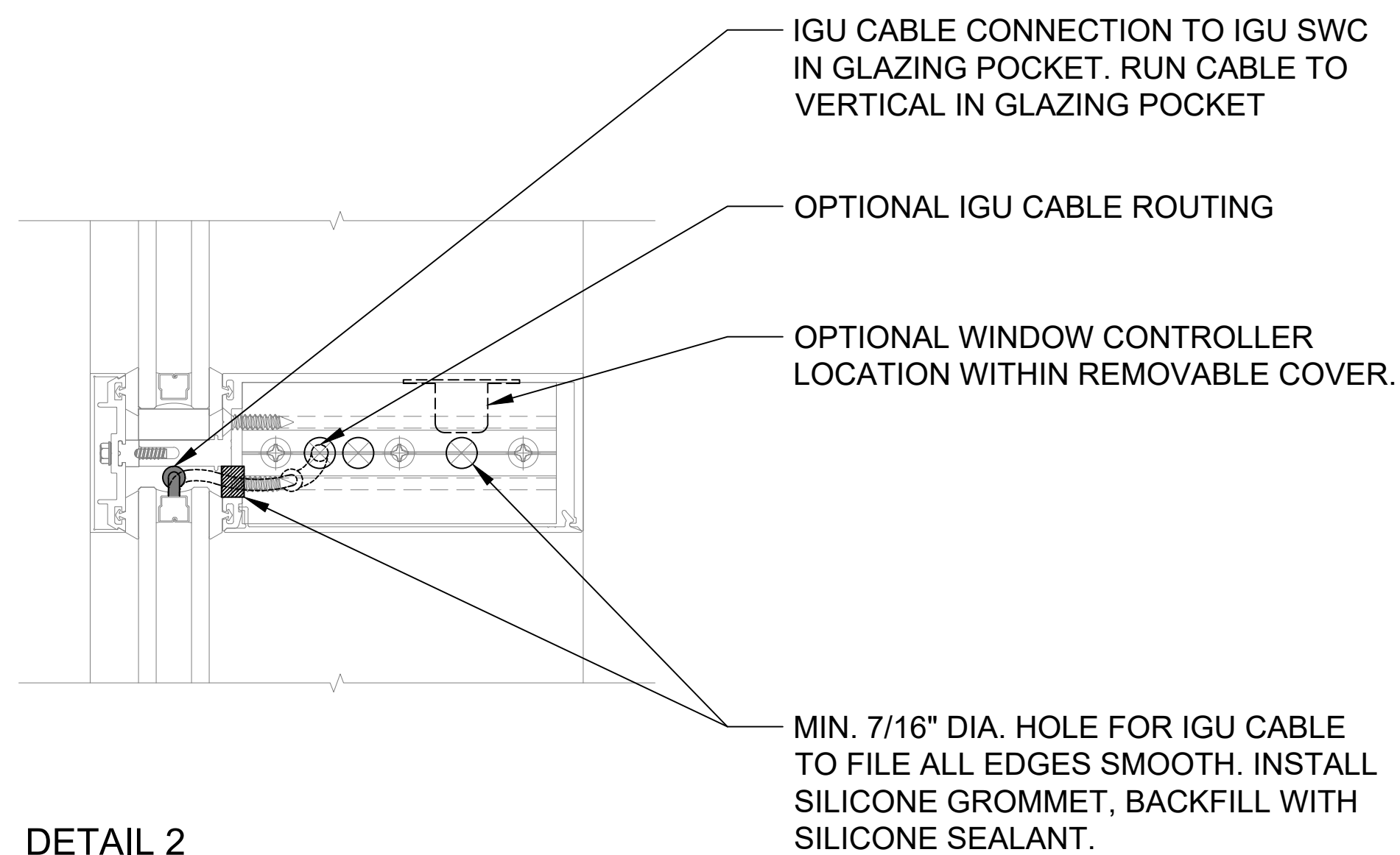
DETAIL 2 HORIZONTAL MULLION
