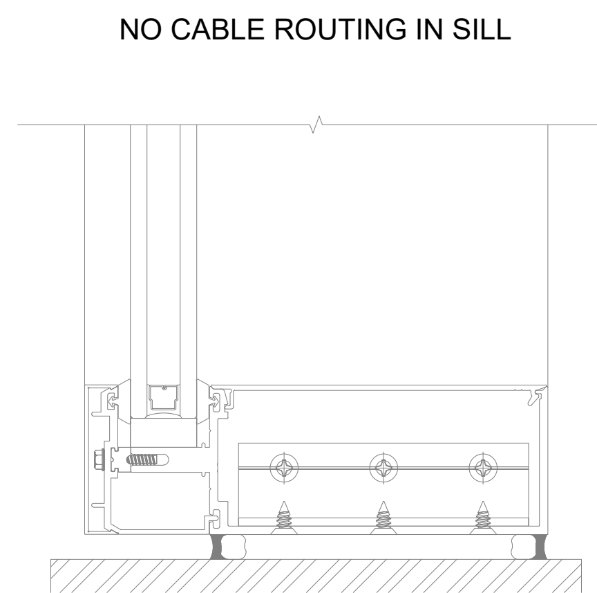
DETAIL 3 SILL
