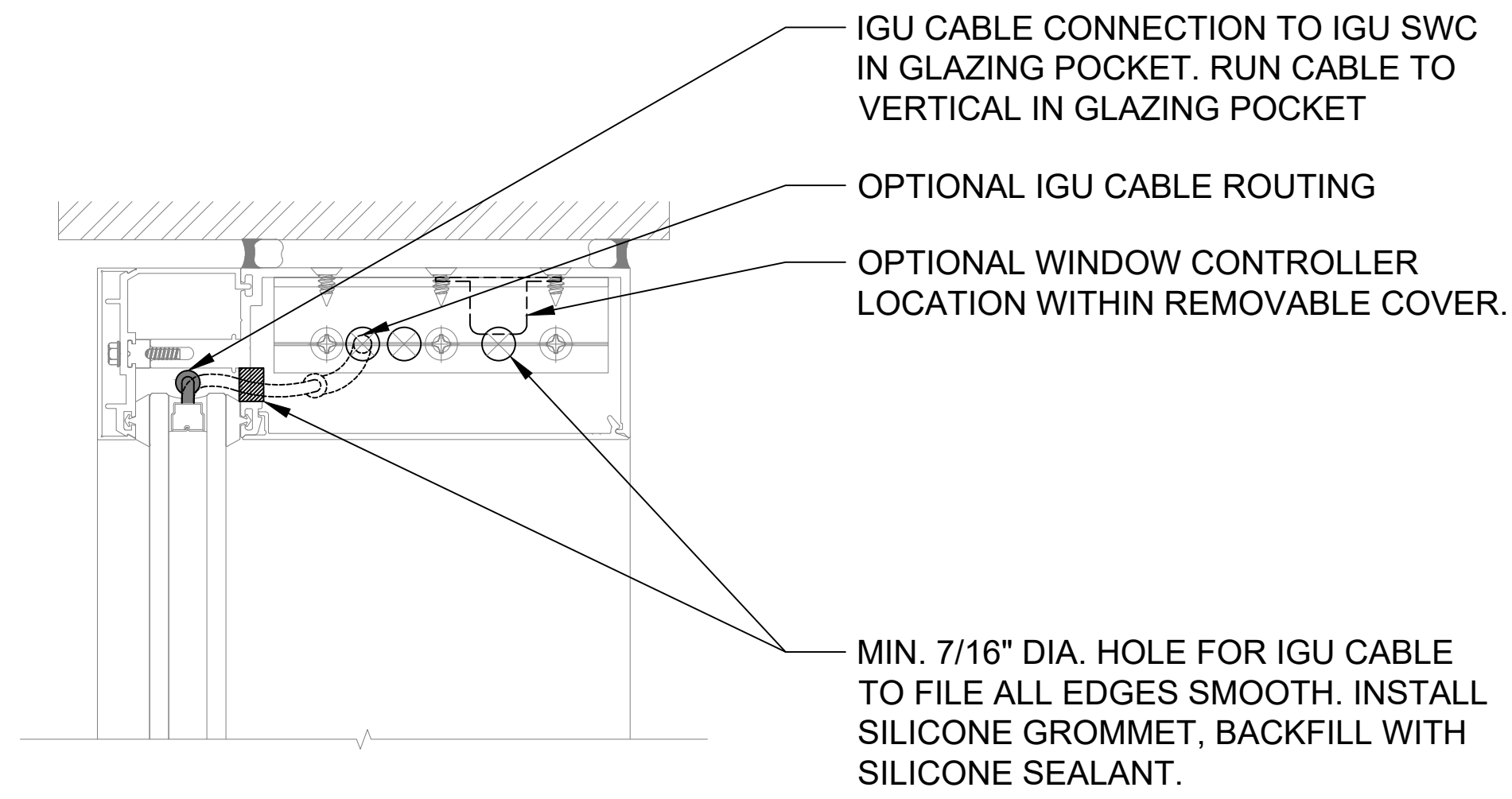
DETAIL 1 HEAD
